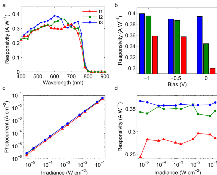
Figure 2. Responsivity measurements. (a) Spectral responsivity at zero bias with 0.1 \text{ mW cm}^{-2} irradiance. The responsivity sharply increases above the bandgap of \text{MAPbI}_3 at 780 \text{ nm} . The responsivity in the green and red ( 560\text{--}660 \text{ nm} ) and in the near-infrared at 750 \text{ nm} is enhanced with the addition of \text{Al}_2\text{O}_3 and PCBM. (b) Responsivities at 0 , -0.5 , and -1 \text{ V} bias at 600 \text{ nm} wavelength with 0.1 \text{ mW cm}^{-2} input irradiance. The interface stack greatly improves the zero bias responsivity with device I3 being bias-insensitive. (c) Photocurrent linearity upon varying the 640 \text{ nm} input irradiance at 0 \text{ V} bias. (d) Responsivity dependence on input irradiance at 640 \text{ nm} with 0 \text{ V} bias. For devices I2 and I3, the input irradiance is flat over 4 decades, corresponding to a dynamic range exceeding 80 \text{ dB} .
