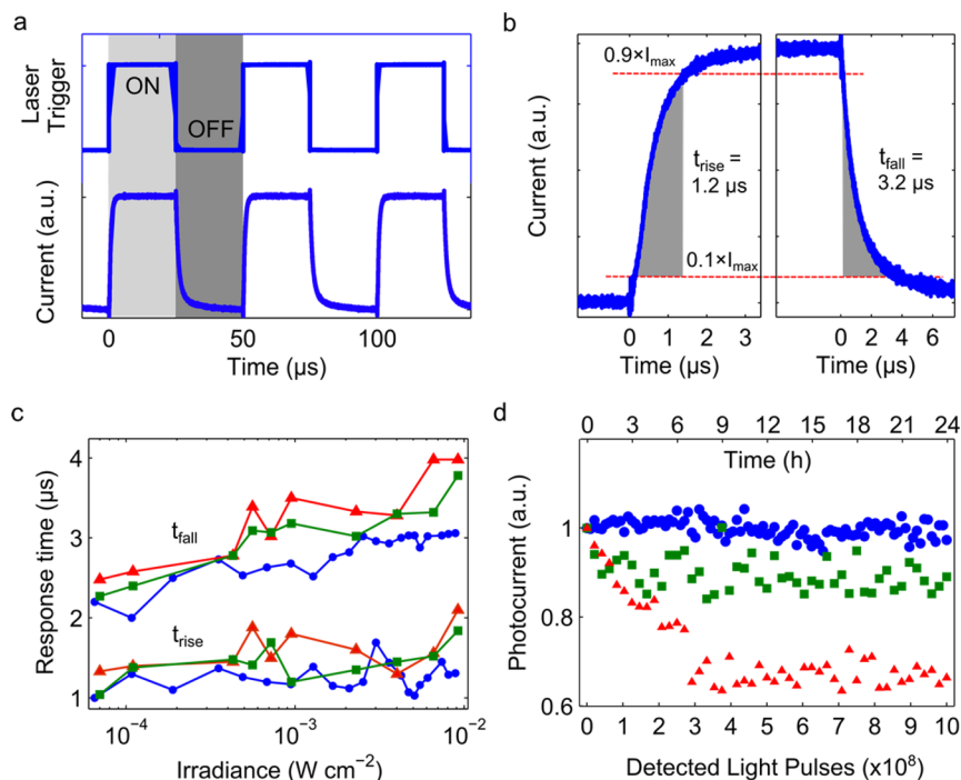
Figure 3. Perovskite photodetector speed at 0 \text{ V} bias. (a) Transient current output of device I3 to a time-varying input light signal ( 640 \text{ nm} , 50 \mu\text{s} period square wave, 20 \text{ mW cm}^{-2} peak-to-peak). (b) Photocurrent rise and fall of device I3 at an input irradiance of 20 \text{ mW cm}^{-2} . Laser pulse is triggered on (rise)/off (fall) at time t = 0 . (c) Rise and fall time dependence on input irradiance for all devices. On average, device I3 is the fastest and least dependent on input irradiance. (d) Device stability in air under continuous illumination ( 640 \text{ nm} , 40 \mu\text{s} period square wave, 100 \mu\text{W cm}^{-2} peak-to-peak). Photocurrent of device I3 is stable over 24 \text{ h} , after the detection of one billion laser pulses. Device I2 experiences an initial decay in photocurrent to 90\% of its initial value, and device I1 experiences gradual photocurrent decay to 60\% of its initial value.
